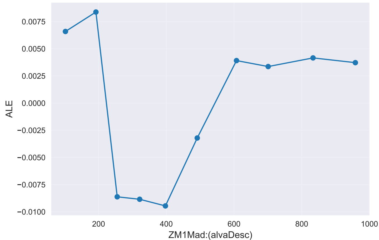
ALE plot: ZM1Mad:(alvaDesc) GradientBoosting__model_specific_best_subset__rank_top_20
