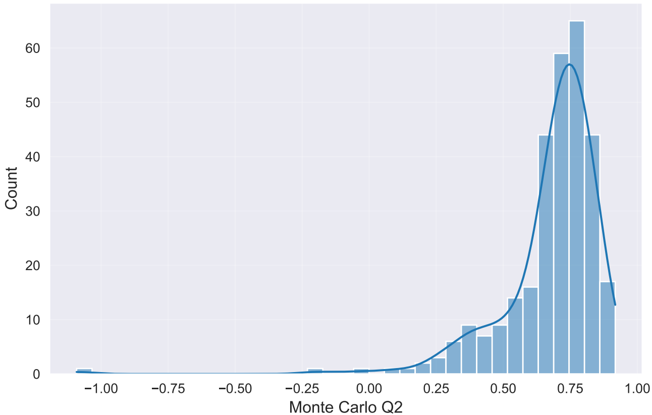
Monte Carlo validation Q2 CatBoost__model_specific_best_subset__rank_top_20
