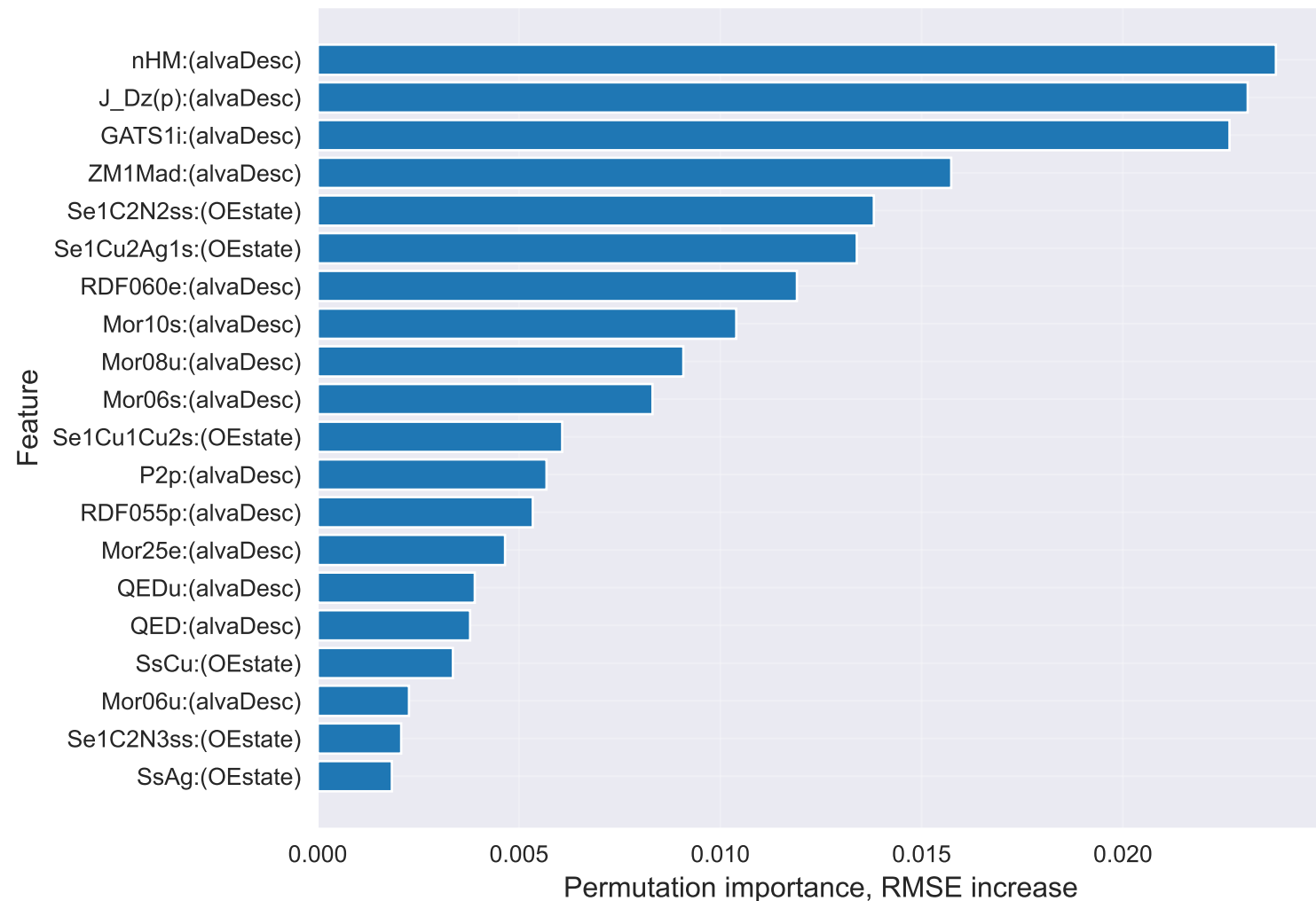
Permutation importance CatBoost__model_specific_best_subset__rank_top_20
