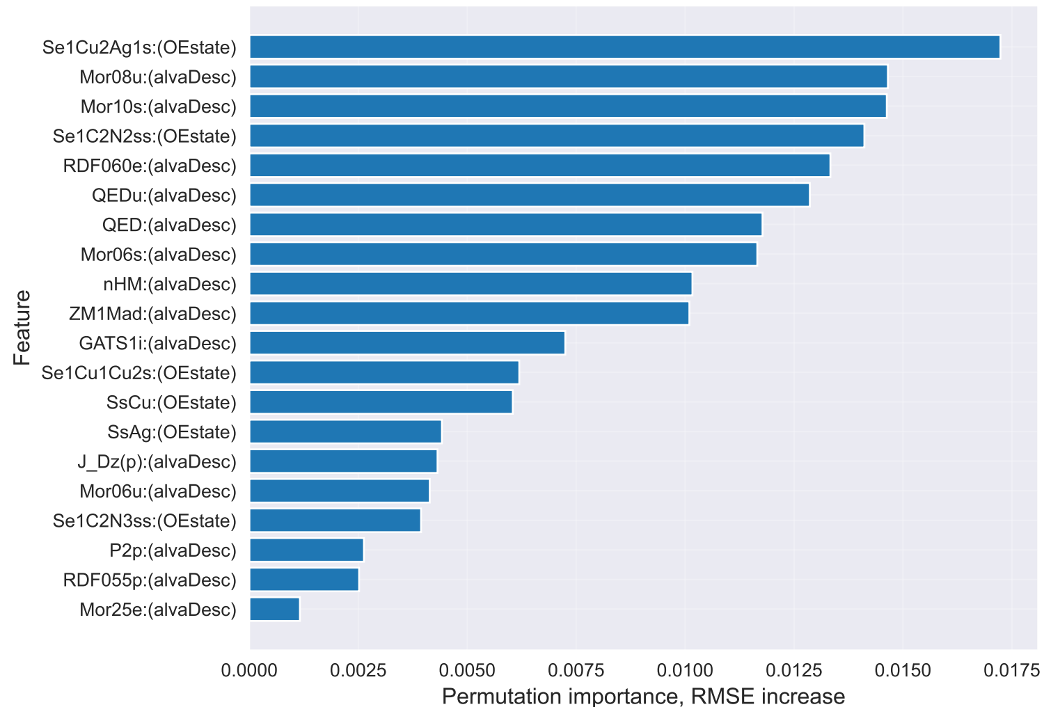
Permutation importance GaussianProcess__model_specific_best_subset__rank_top_20
