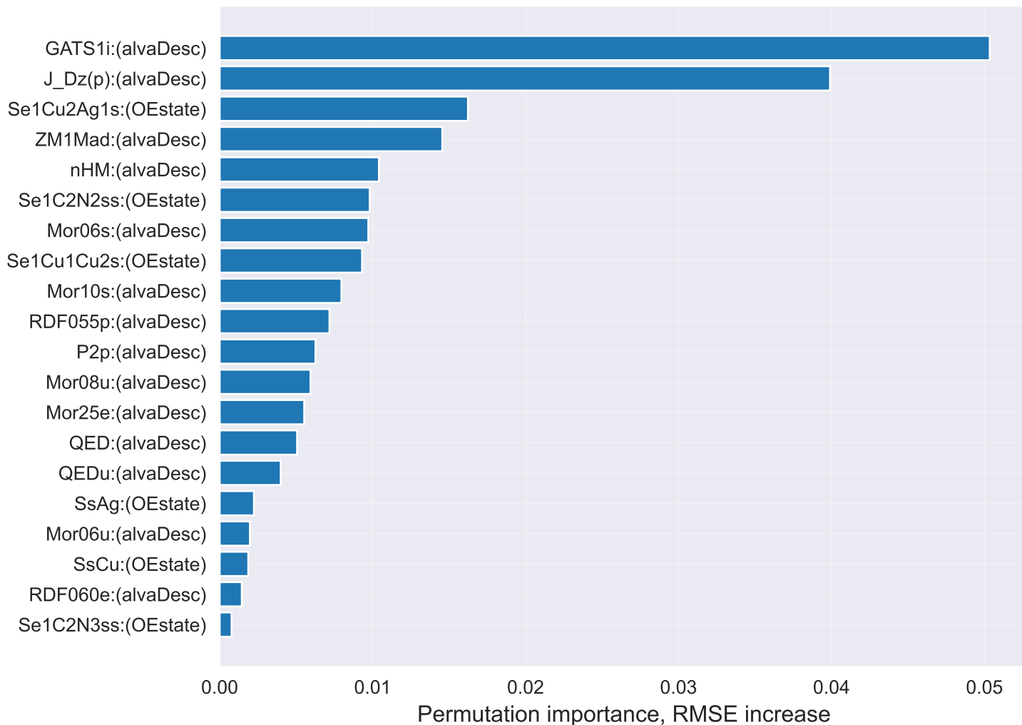
Permutation importance GradientBoosting__model_specific_best_subset__rank_top_20
