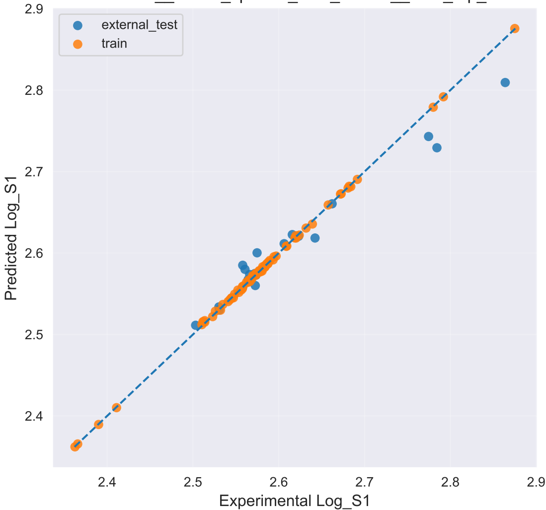
Predicted vs Experimental CatBoost__model_specific_best_subset__rank_top_20
