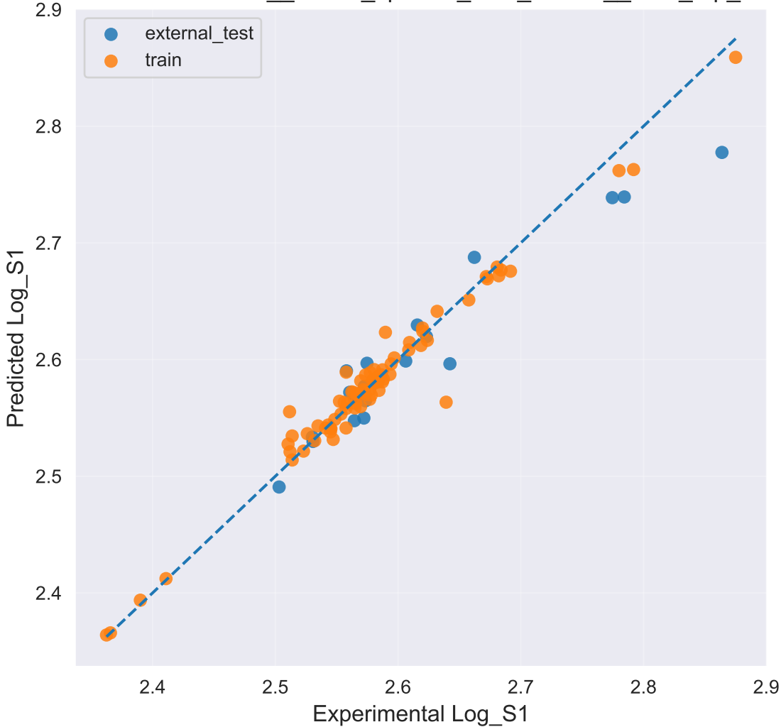
Predicted vs Experimental GaussianProcess__model_specific_best_subset__rank_top_20
