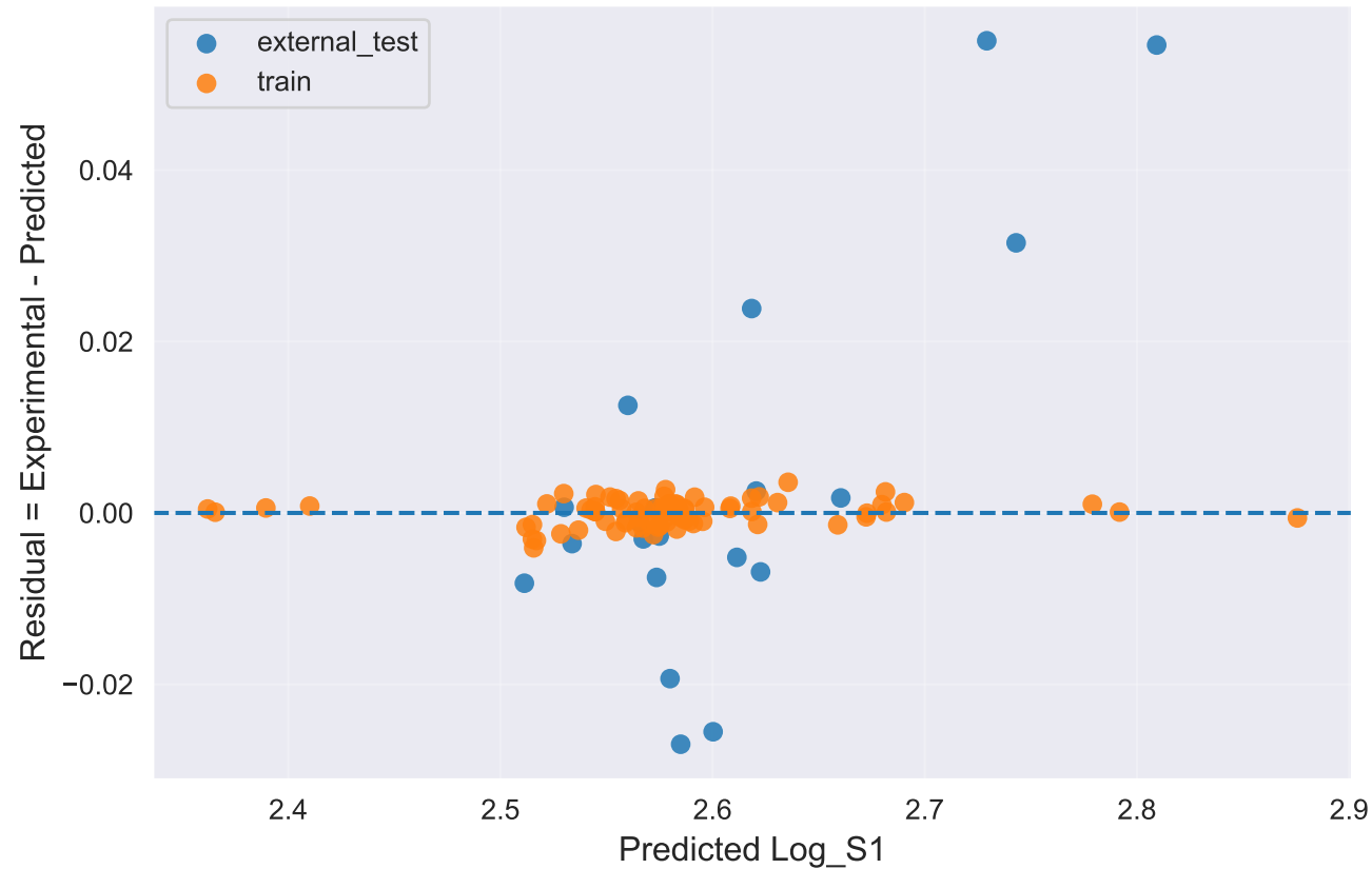
Residual plot CatBoost__model_specific_best_subset__rank_top_20
