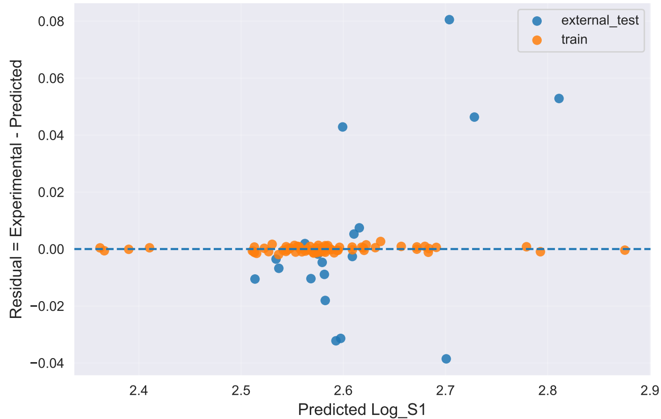
Residual plot GradientBoosting__model_specific_best_subset__rank_top_20
