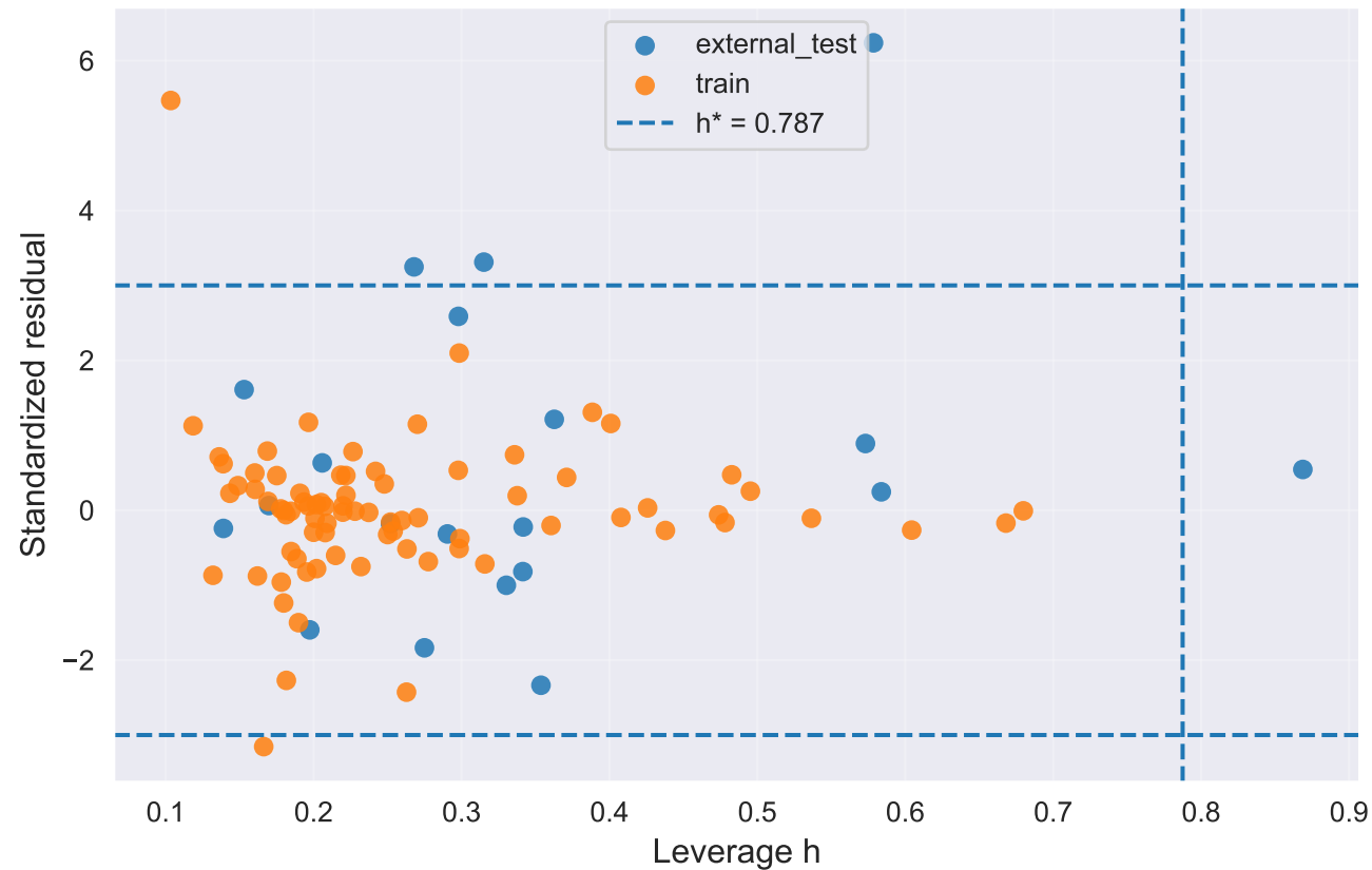
Williams plot GaussianProcess__model_specific_best_subset__rank_top_20
