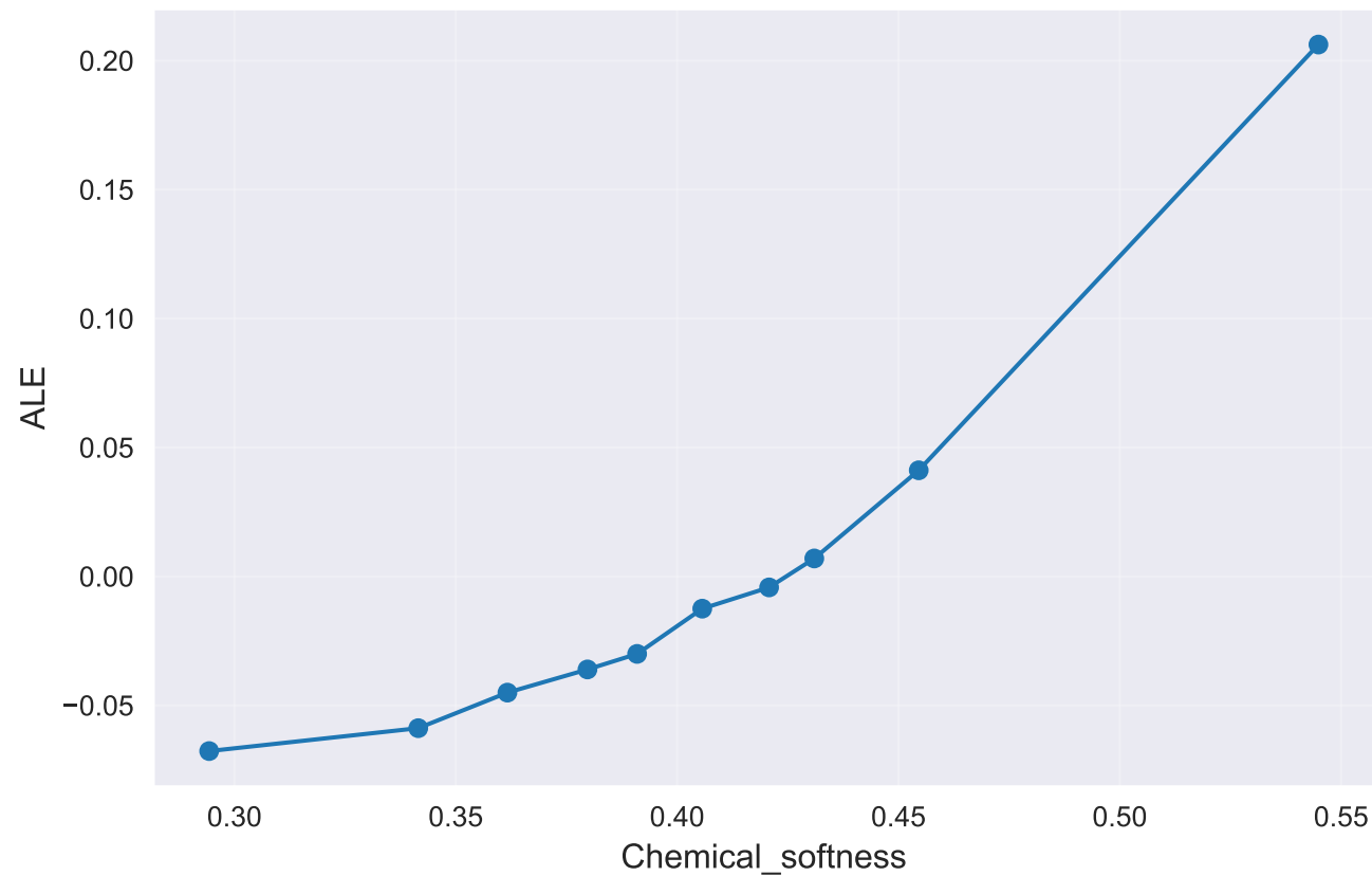
ALE plot: Chemical_softness GaussianProcess__global_robust_subset__rank_top_10
