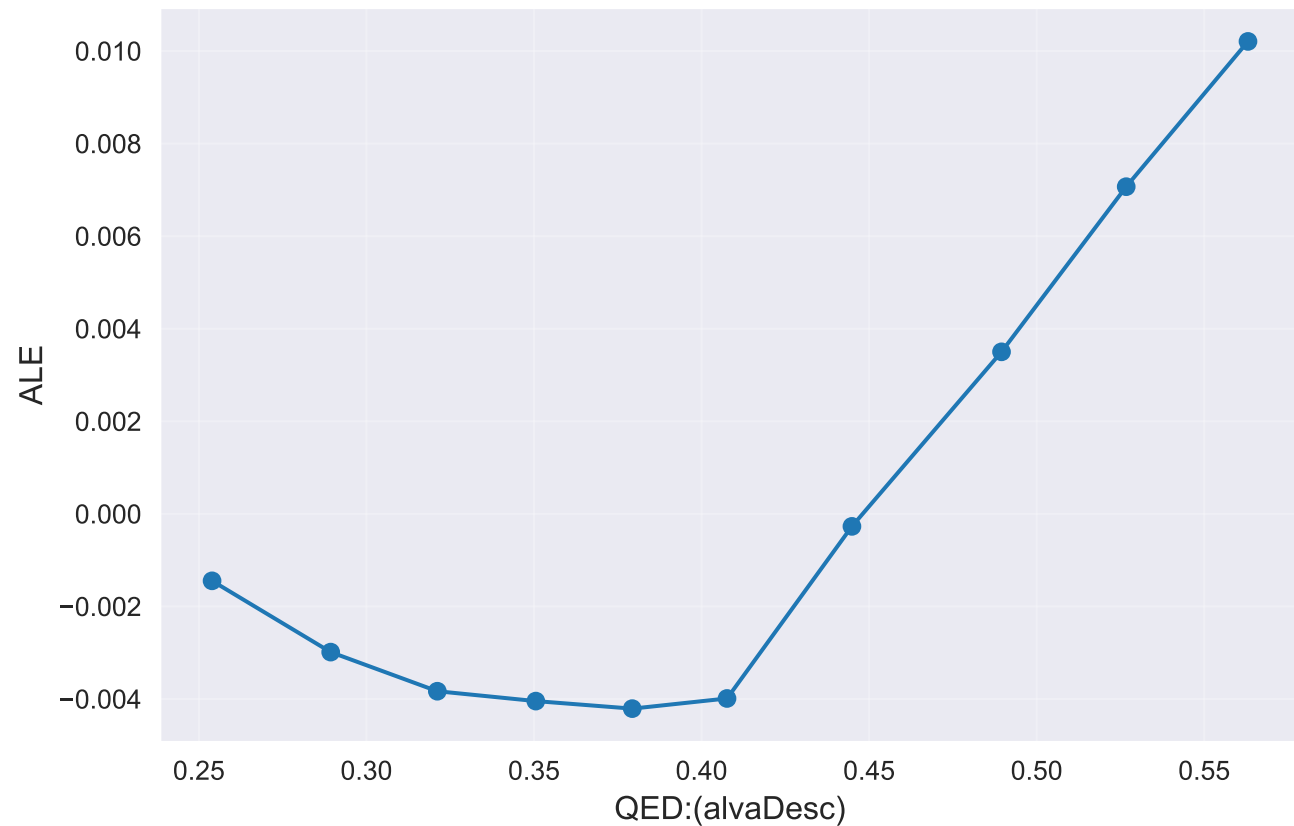
ALE plot: QED:(alvaDesc) GaussianProcess__global_robust_subset__rank_top_10
