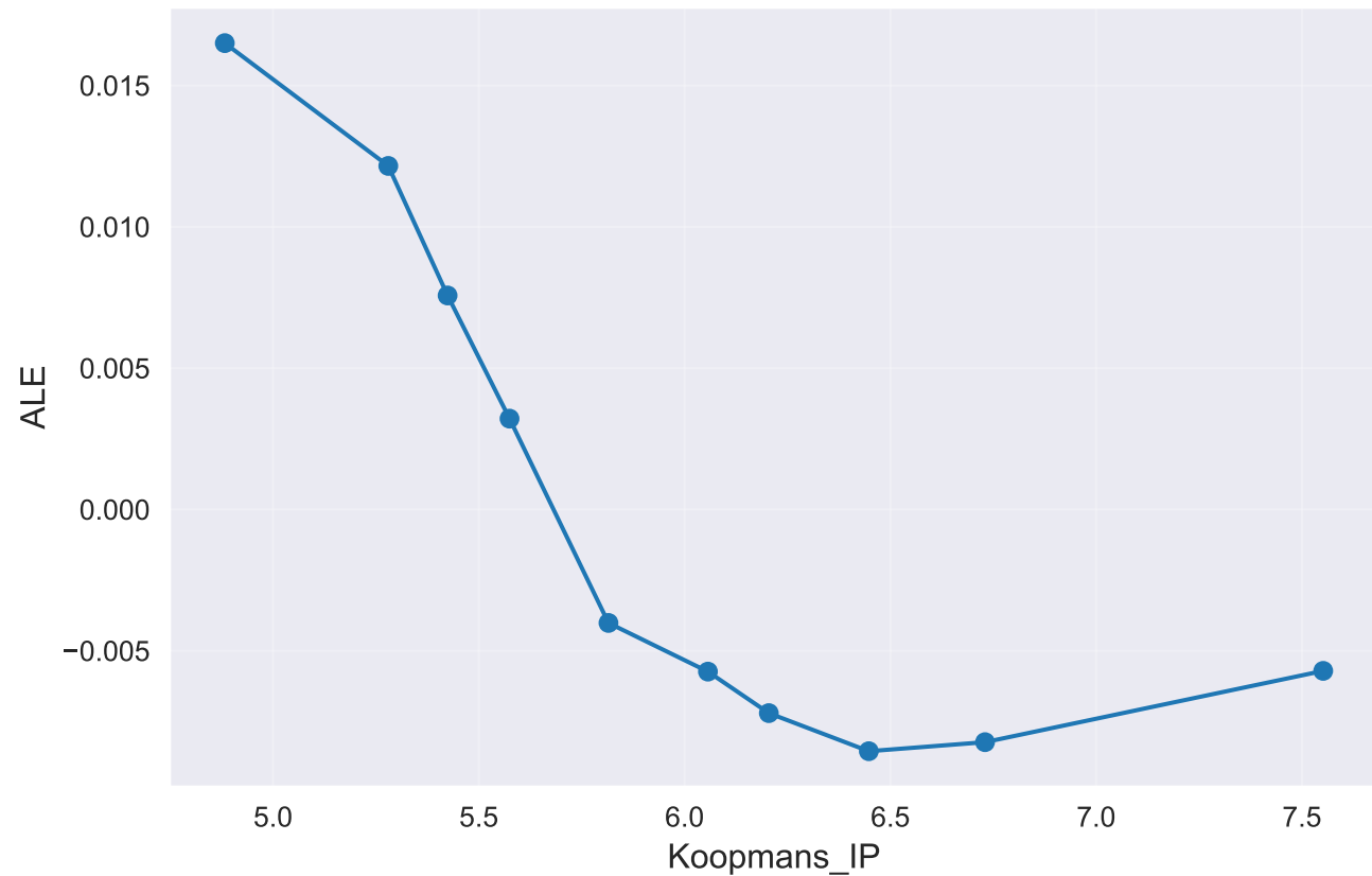
ALE plot: Koopmans_IP GaussianProcess__model_specific_best_subset__rank_top_8
