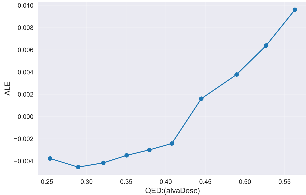
ALE plot: QED:(alvaDesc) GaussianProcess__model_specific_best_subset__rank_top_8
