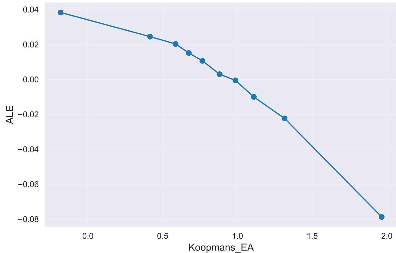
ALE plot: Koopmans_EA Ridge__model_specific_best_subset__rfe_subset
