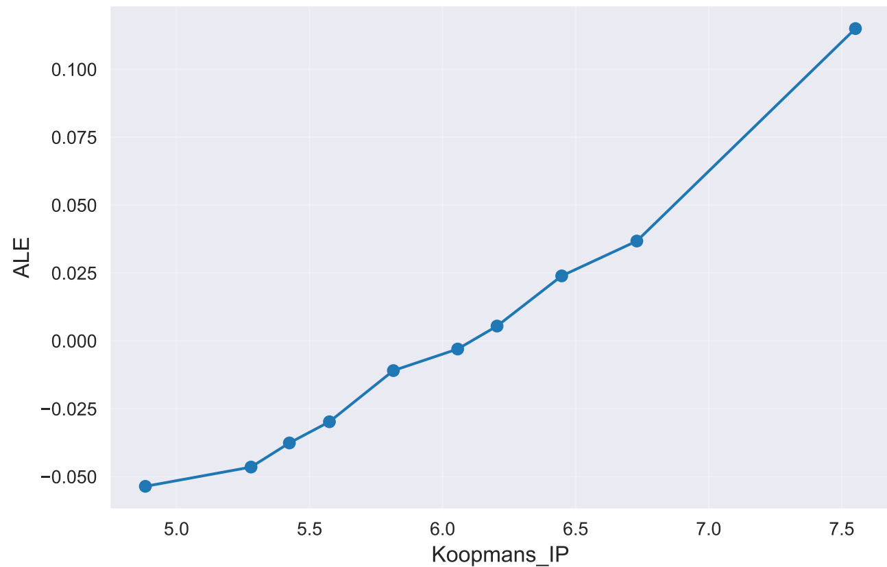
ALE plot: Koopmans_IP Ridge__model_specific_best_subset__rfe_subset
