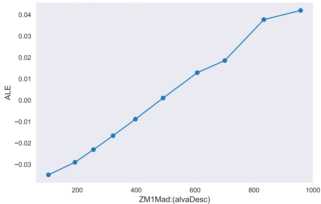
ALE plot: ZM1Mad:(alvaDesc) Ridge__model_specific_best_subset__rfe_subset
