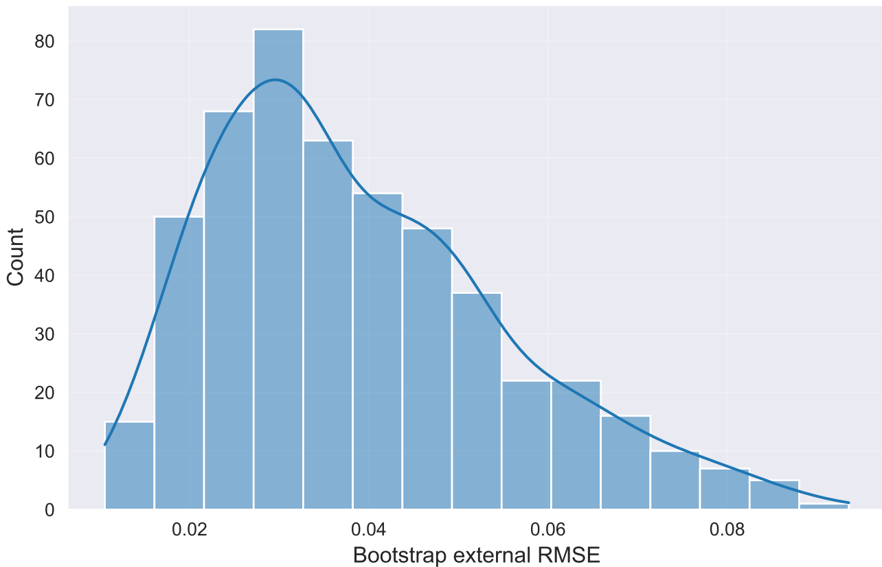
Bootstrap external RMSE GaussianProcess__model_specific_best_subset__rank_top_8
