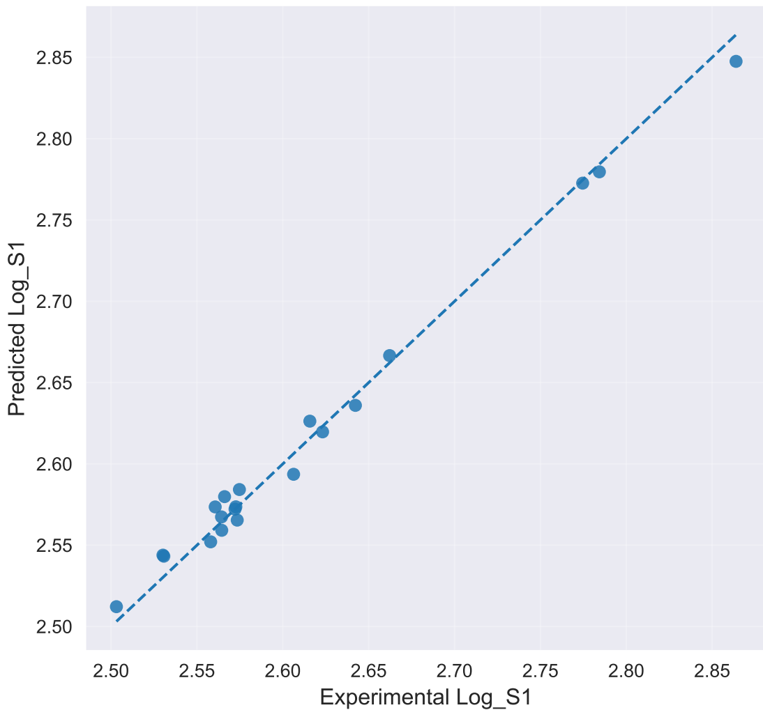
External test ensemble weighted_average_prediction
