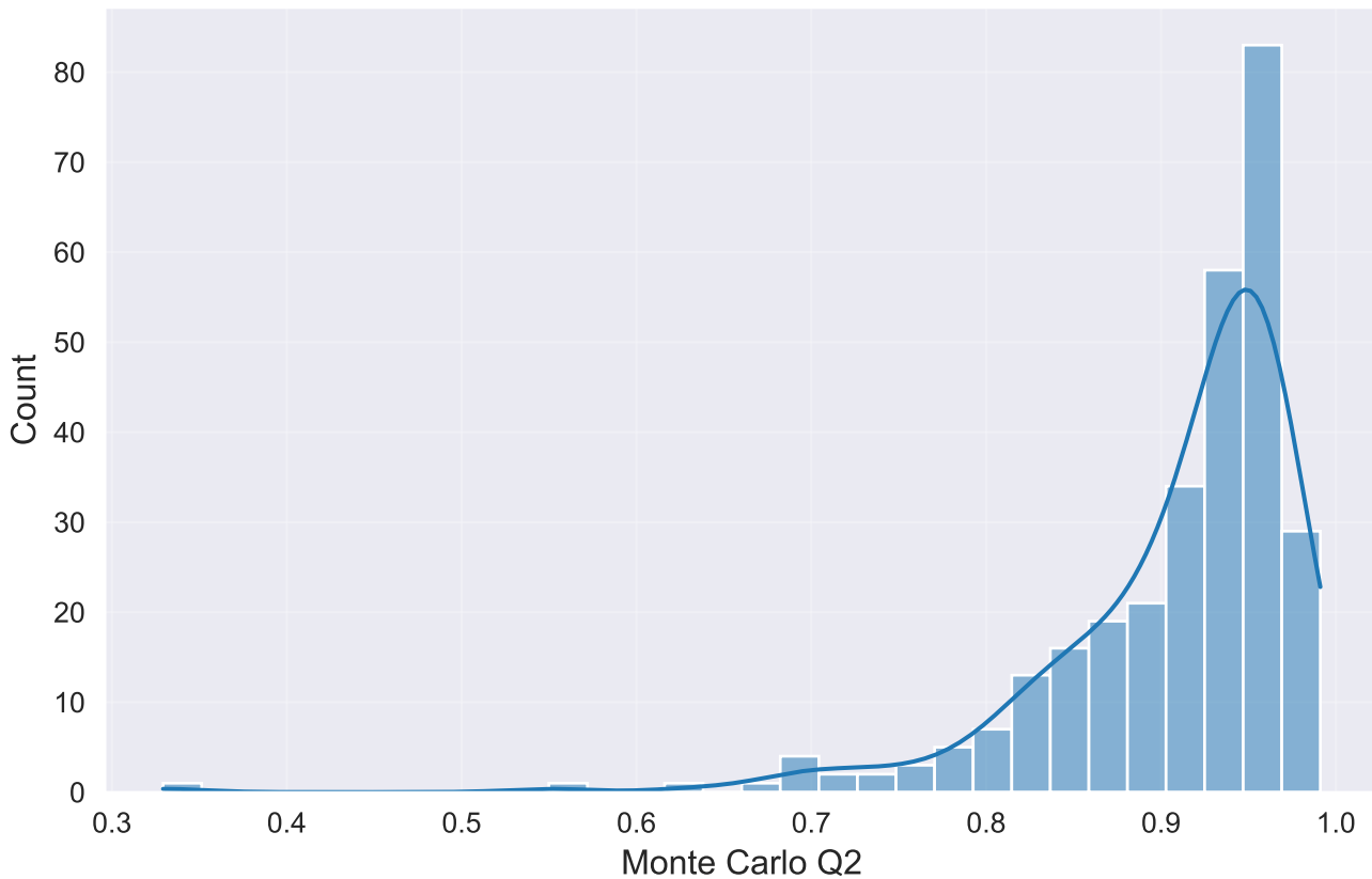
Monte Carlo validation Q2 Ridge__model_specific_best_subset__rfe_subset
