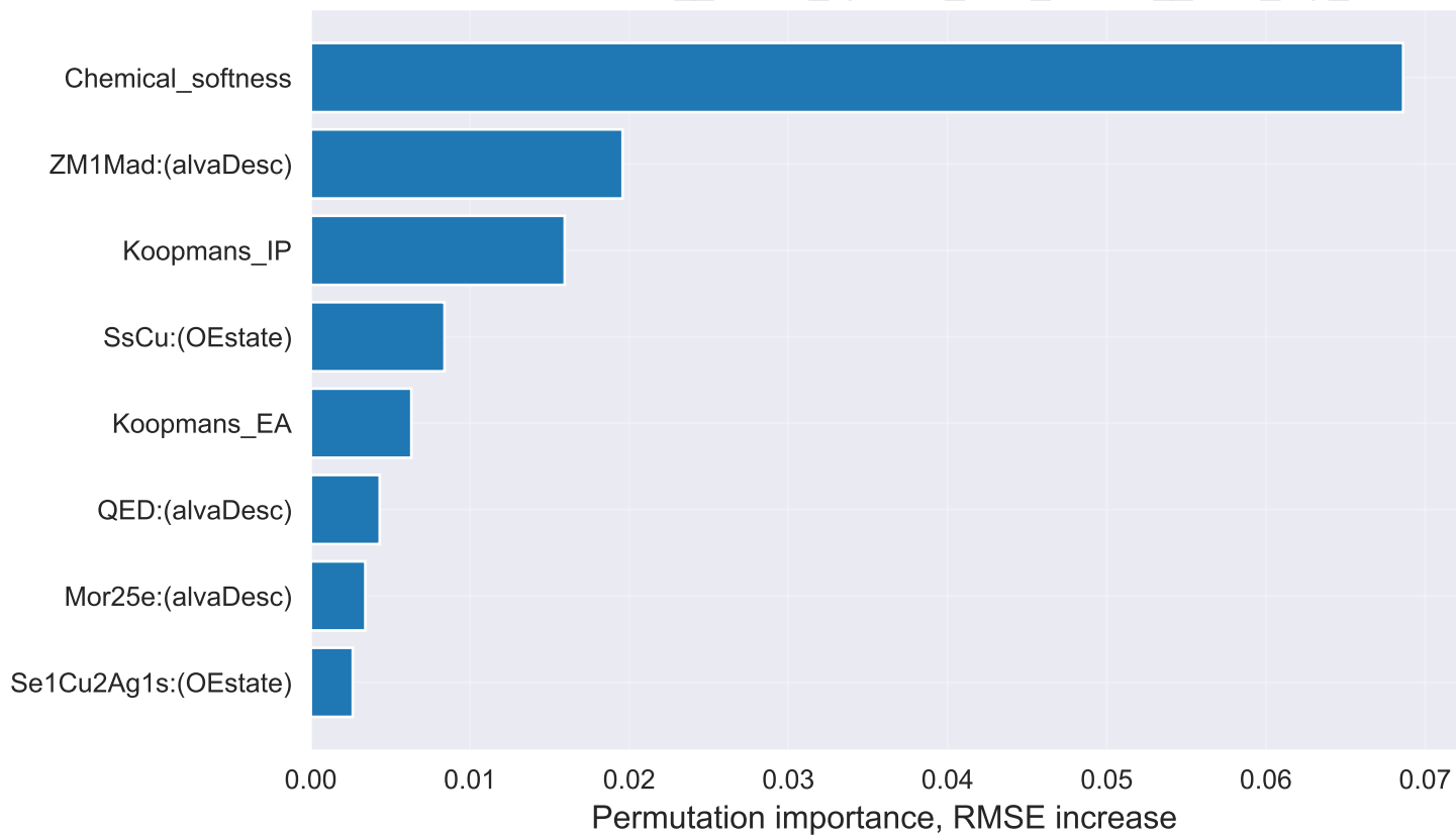
Permutation importance GaussianProcess__model_specific_best_subset__rank_top_8
