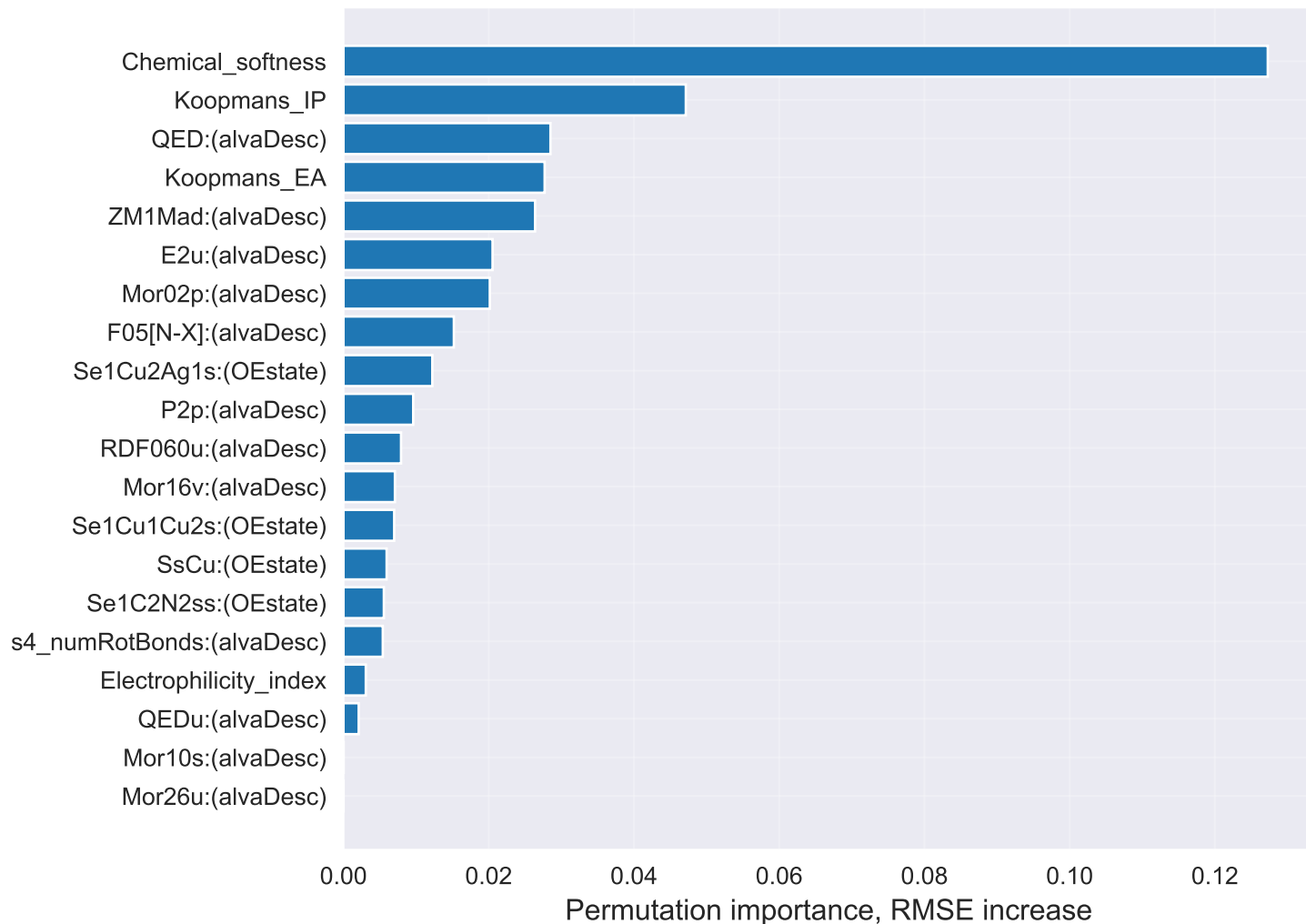
Permutation importance Ridge__model_specific_best_subset__rfe_subset
