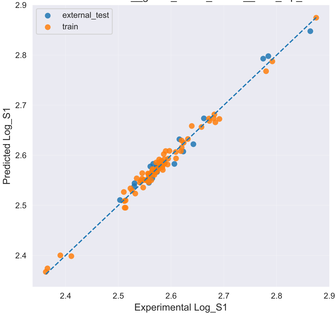
Predicted vs Experimental GaussianProcess__global_robust_subset__rank_top_10
