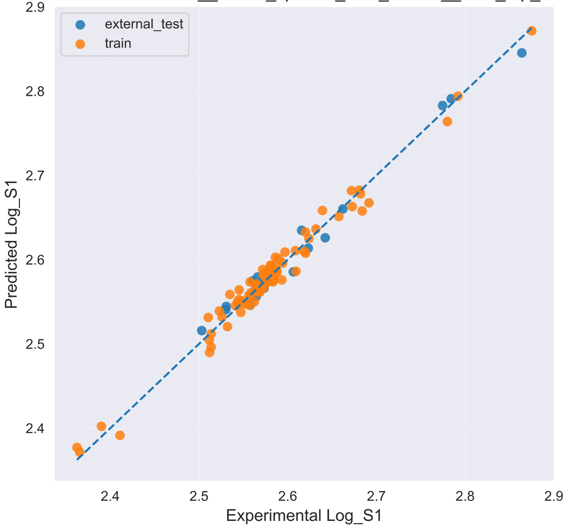
Predicted vs Experimental GaussianProcess__model_specific_best_subset__rank_top_8
