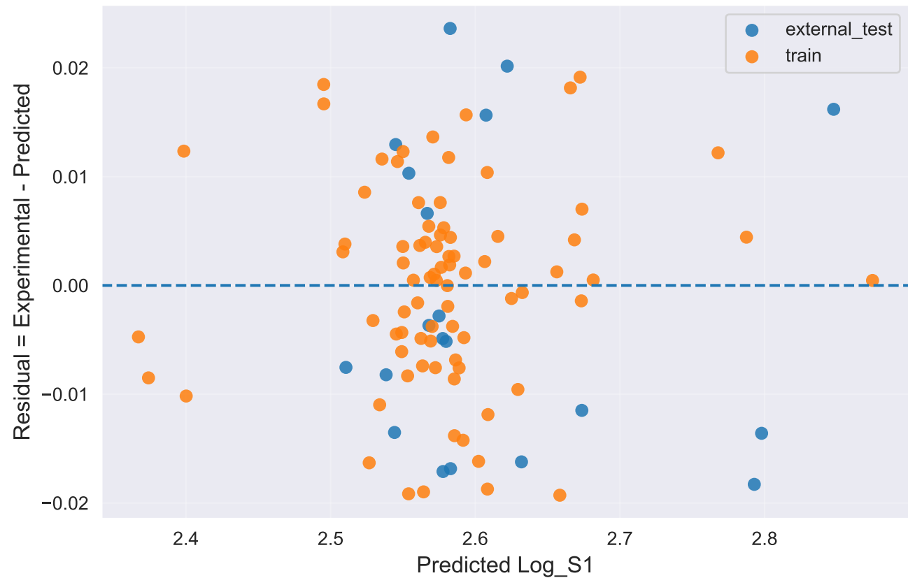
Residual plot GaussianProcess__global_robust_subset__rank_top_10
