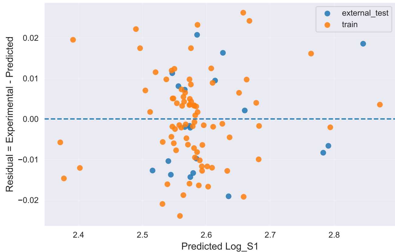
Residual plot GaussianProcess__model_specific_best_subset__rank_top_8
