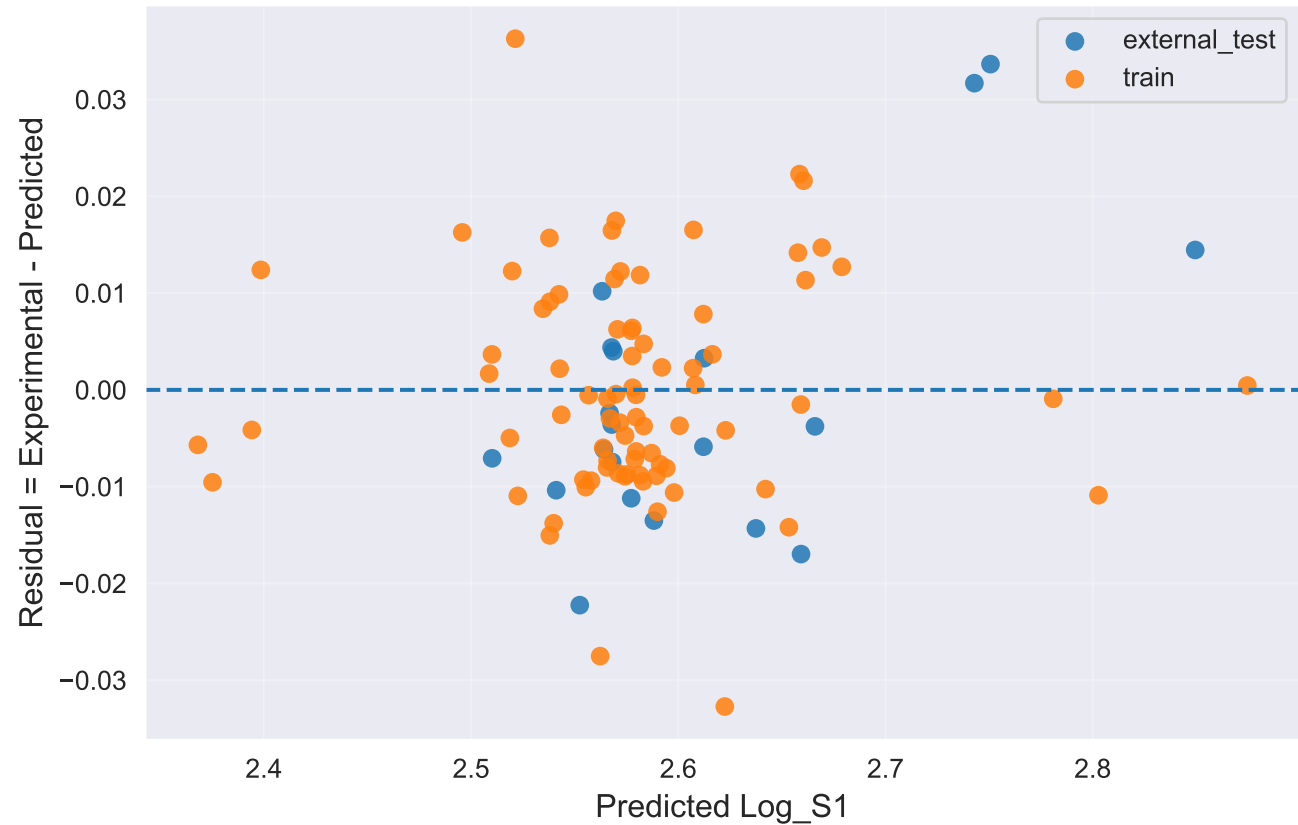
Residual plot Ridge__model_specific_best_subset__rfe_subset
