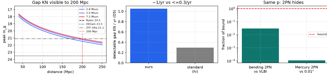
Fig 69 — BU: O5 detectability + GR-battery 2PN margins
