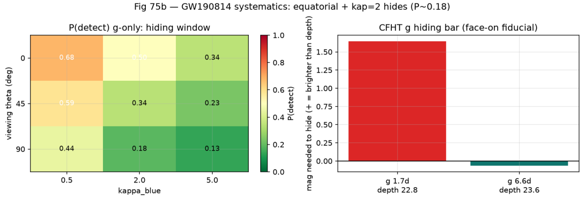
Figure 12: GW190814 analytic systematics (round 4; full POSSIS queued, D7). Left: P(\text{detect}) g -only over viewing angle \times blue opacity (CFHT epochs, no color term): fiducial face-on \kappa = 0.5 gives 0.68; equatorial + lanthanide-mixed ( \kappa_{\text{blue}} = 2 ) drops to \sim 0.18 . Right: face-on hiding bar per CFHT g epoch ( g 1.7 d needs \sim 1.6 mag). Module massgaps .
