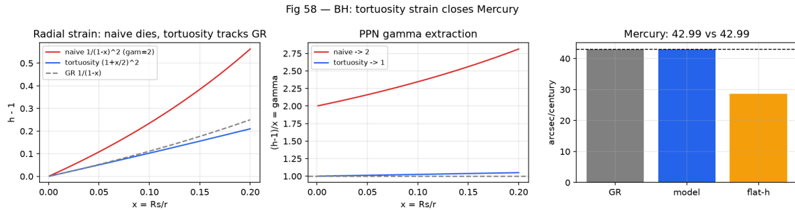
Fig 58 — BH: tortuosity strain closes Mercury
