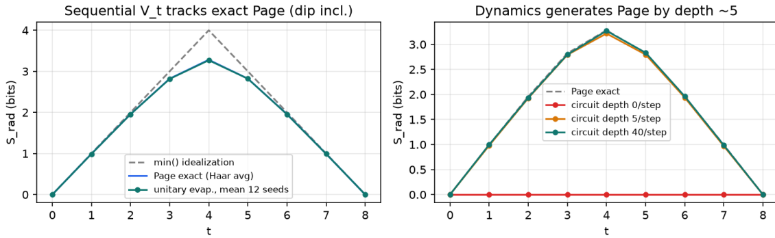
Fig 74 — D2: unitary evaporation ( V \hat{d} V = I , S from \rho_{\text{rad}} )
