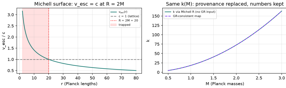
Fig 3b — BM2: R_s = 2M from entropic Newton + c (metric never imported)
