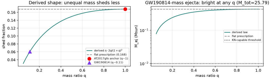
Fig 68b — BU2: graph-derived shedding shape (O5 adjudicates flat vs shaped)
