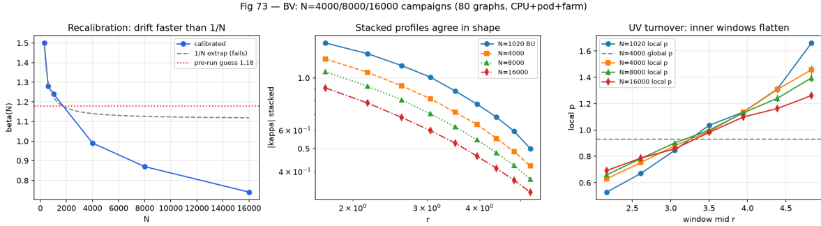
Figure 12: N-scale campaigns: \beta(N) recalibration drifts faster than 1/N (left); stacked |\kappa|(r) profiles agree in shape across 1020–16000 (middle); local- p windows show the UV turnover with SEM error bars (right). 80 graphs per production row. shellscale , sinkor .
