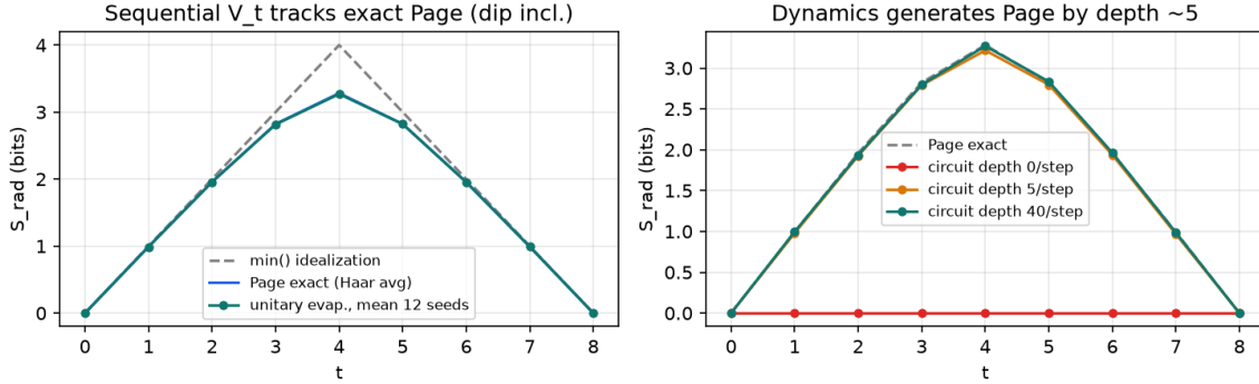
Fig 74 — D2: unitary evaporation ( V \hat{=} V=I , S from \rho_{\text{rad}} )
