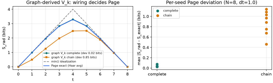
Fig 74b — D1 graph instance: V_k from adjacency ( V^d V=l , S from \rho_{\text{rad}} )
