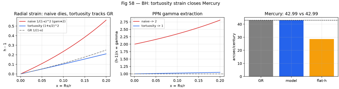
Figure 3: Gravity battery II: naive strain gives \gamma = 2 (excluded); tortuosity h = (1 + x/2)^2 gives \gamma = 1 exactly and Mercury 42.99''/\text{cy} by direct geodesic integration. strain.
