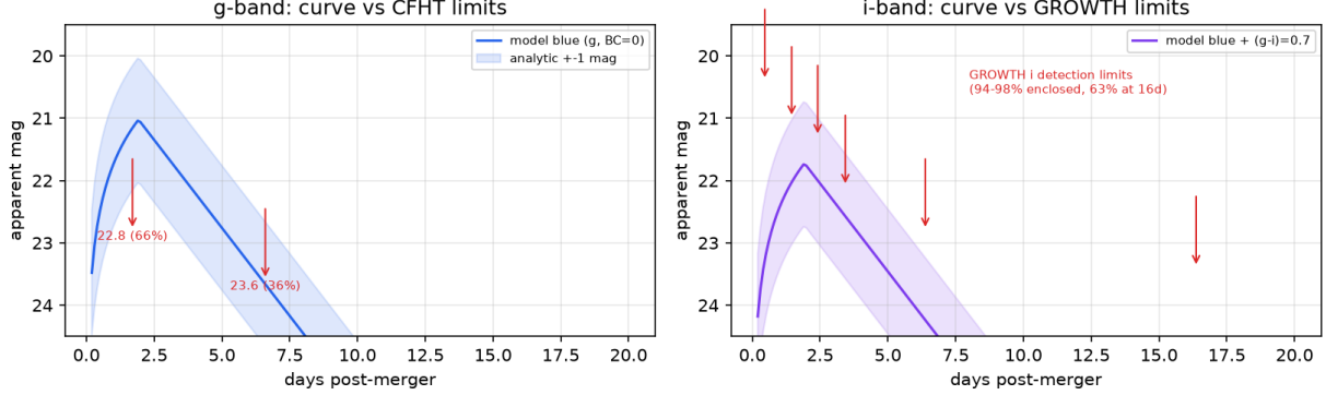
Figure 5: Epoch-level GW190814 audit: model blue light curve ( \pm 1 mag analytic band) against CFHT g-band limits (left, color-free) and GROWTH i-band detection limits (right, g - i = 0.7 systematic). Combined P(\text{detect}) \approx 0.68 (robust) to 0.88 (color-conditional): tension, not exclusion. Module massgaps .
