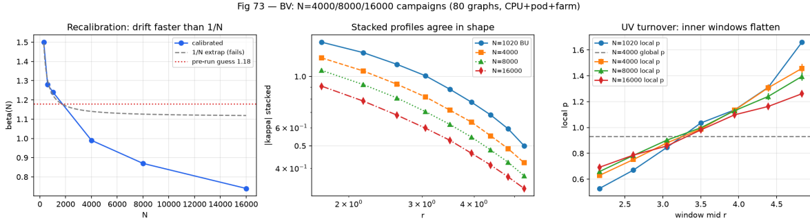
Figure 8: N-scale campaigns: \beta(N) recalibration drifts faster than 1/N (left); stacked |\kappa|(r) profiles agree in shape across 1020–16000 (middle); local- p windows show the UV turnover with SEM error bars (right). 80 graphs per production row. shellscale , sinkor .
