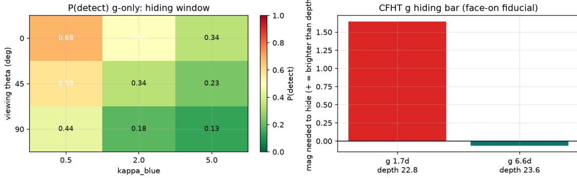
Fig 75b — GW190814 systematics: equatorial + kap=2 hides ( P \sim 0.18 )
