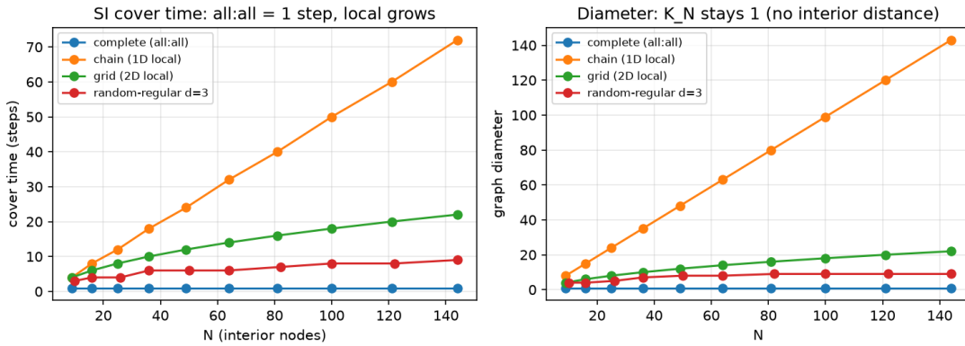
Figure 2: SI cover time and diameter: all:all stays at 1 while local baselines grow. Finite-speed circuits (supplement §3) promote this to t_* \sim \log N .
