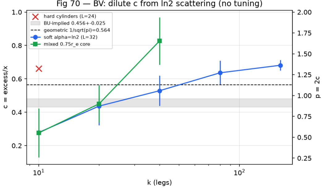
Figure 3: BV tortuosity from ln2 scattering: dilute c = 0.44\text{--}0.60 with zero tuning against the BU-implied 0.456 \pm 0.025 band and the geometric 1/\sqrt{\pi} line. Right axis shows p = 2c . Hard cylinders (red \times ) overshoot; soft and mixed modes agree. uvscatter .
