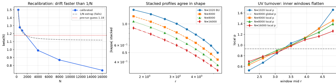
Fig 73 — BV: N=4000/8000/16000 campaigns (80 graphs, CPU+pod+farm)
