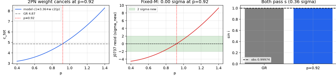
Fig 66 — BU: 2PN cancellation at p=0.92 (J0737 0.00 sigma)
