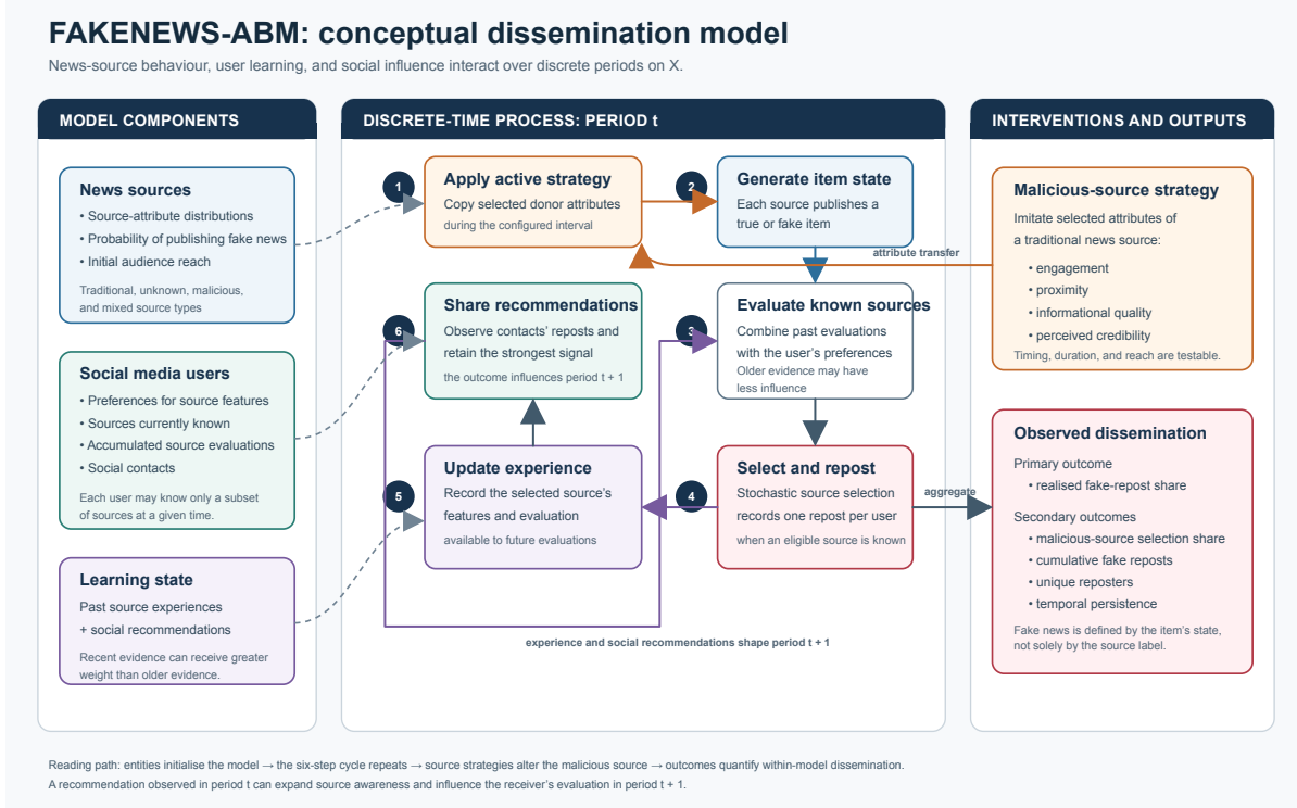
Figure 2: Conceptual structure of the ABM. One source-period publication state is generated before user decisions and is shared by all users who select that source in the period.
