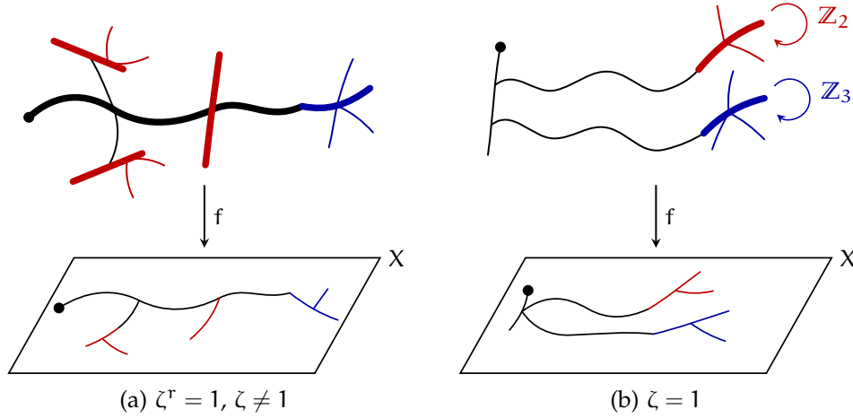
FIGURE 4. The components of \tilde{M}_{0,1}(X, \beta) , due to You-Cheng.
