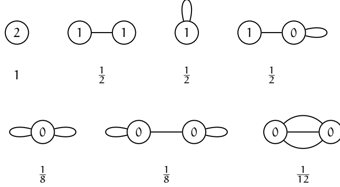
FIGURE 7. The seven stable graphs of genus two with no legs, labelled by the genera of the vertices and weighted by \frac{1}{|\text{Aut } \Gamma|} . On the slides each vertex was drawn as its Riemann surface component.
