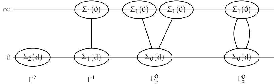
FIGURE 6. The four non-constant localization graphs in genus two, with each vertex drawn as its Riemann surface component.
