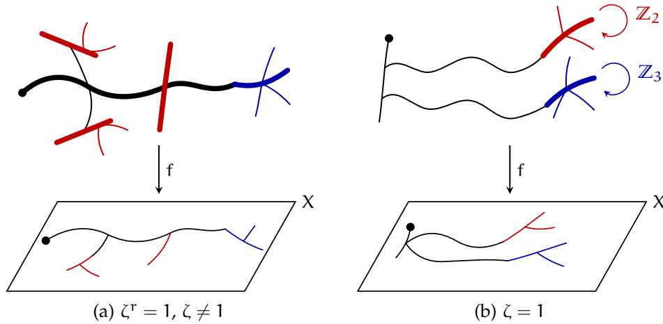
FIGURE 4. The components of \bar{M}_{0,1}(X, \beta) , due to You-Cheng.
