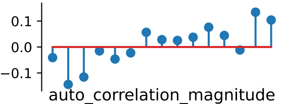
std+skew+kurtosis recon
