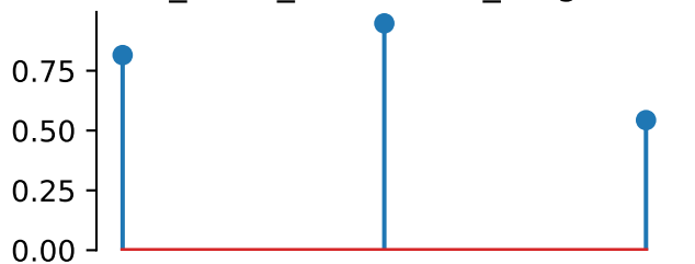
cross_scale_correlation_magnitude
