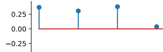
cross_scale_correlation_magnitude
