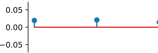
cross_scale_correlation_real
