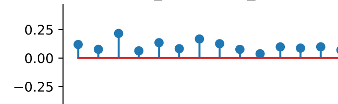
cross_scale_correlation_real
