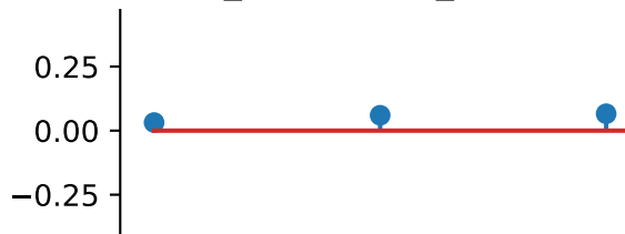
cross_orientation_correlation_magnitude
