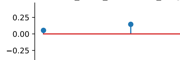
cross_scale_correlation_magnitude
