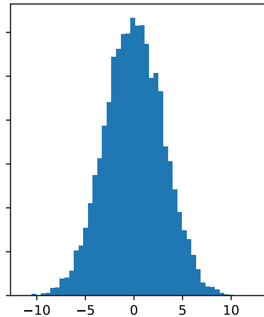
\sigma=3 Variance: 9.0795
