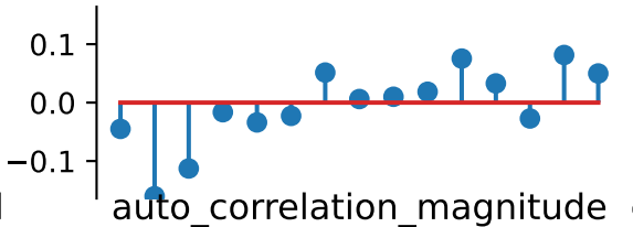
std+skew+kurtosis recon
