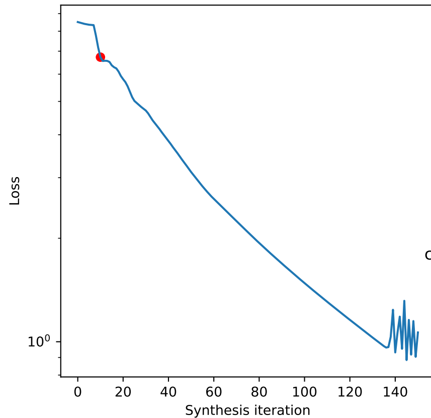
Representation error
