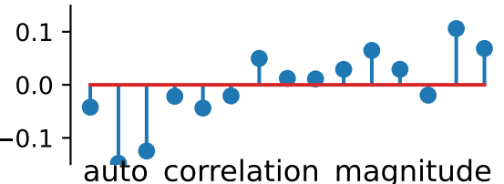
std+skew+kurtosis recon
