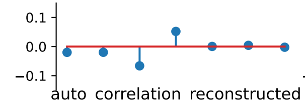
pixels+var_highpass
