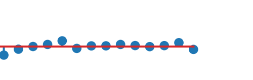
orientation_correlation_magnitude
