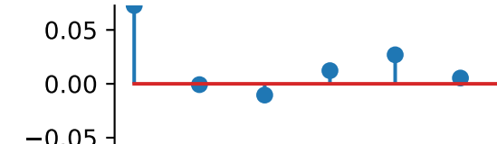
auto_correlation_reconstructed
