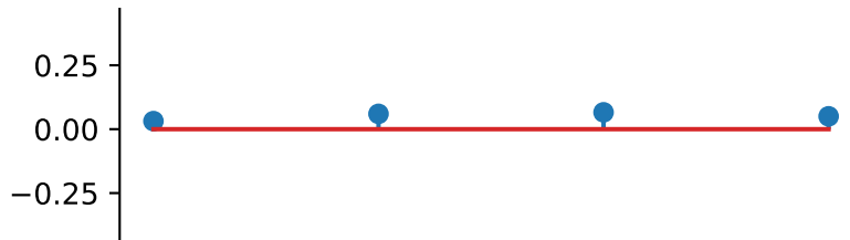
cross_orientation_correlation_magnitude
