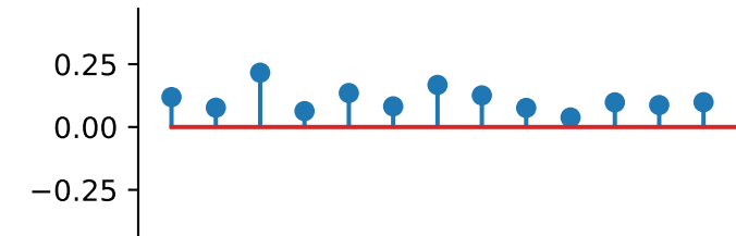
cross_scale_correlation_real
