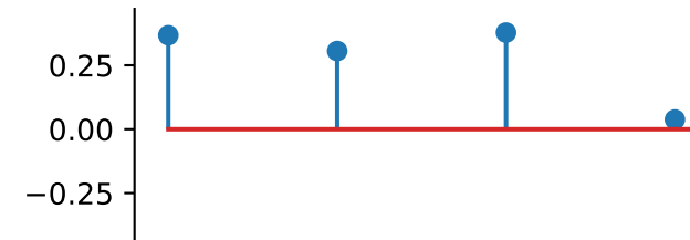
cross_scale_correlation_magnitude
