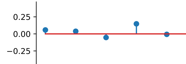
auto_correlation_reconstructed
