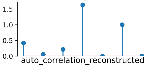
pixels+var_highpass
